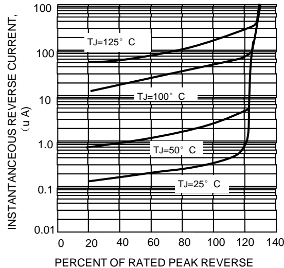
FIG.5-TYPICAL REVERSE CHARACTERISTICS
