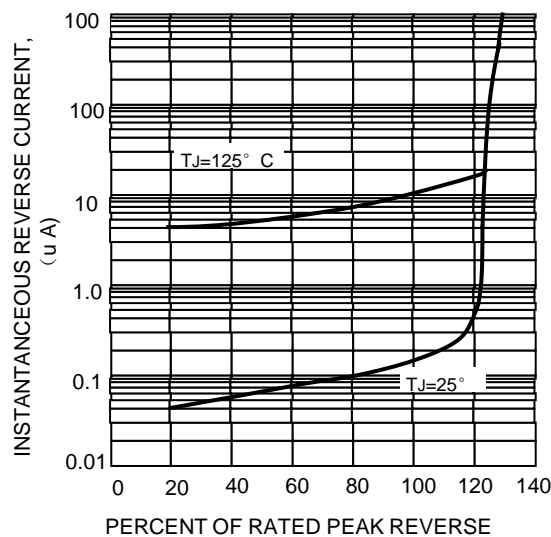
FIG.5-TYPICAL REVERSE
