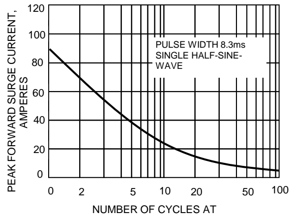
FIG.2-MAXIMUM NON-REPETITIVE SURGE
