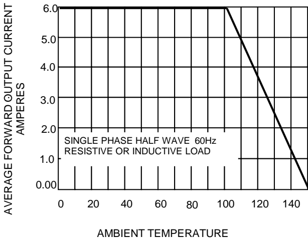
FIG.1-FORWARD DERATING CURRENT
